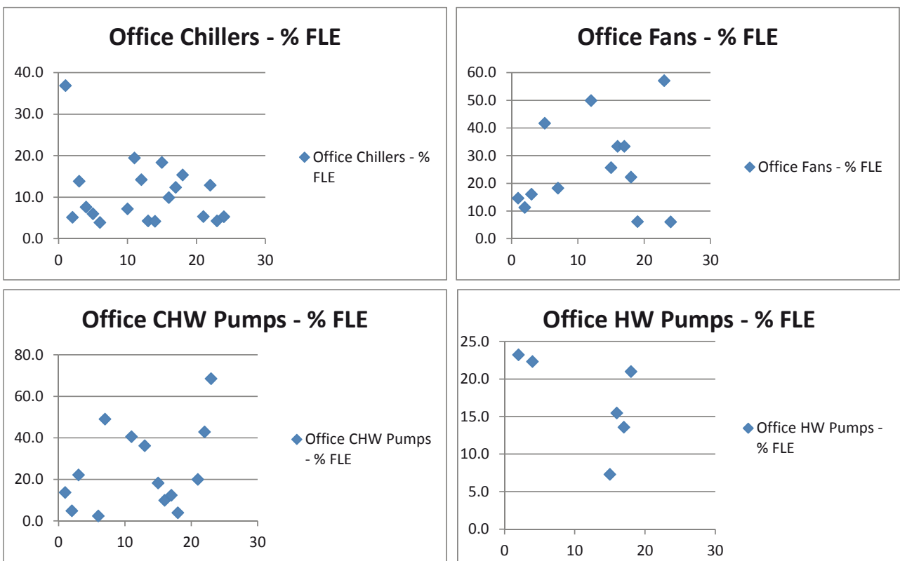
Figure 4. Measured average annual power demand by HVAC component as a percentage of the Full Load Equivalent for HARMONAC Case Study systems.
